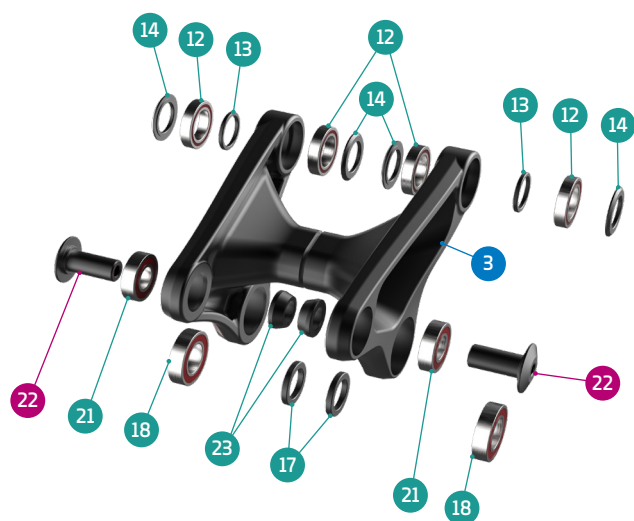
DETAIL 01
