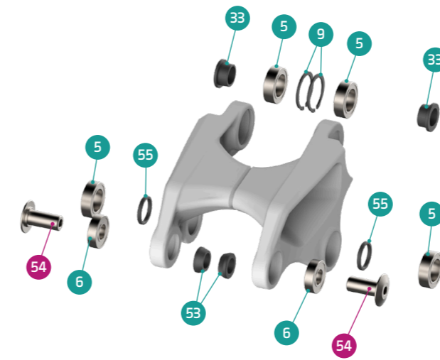
DETAIL 01
