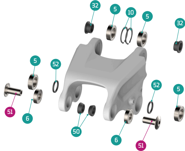
DETAIL 01
