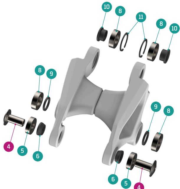
DETAIL 01
