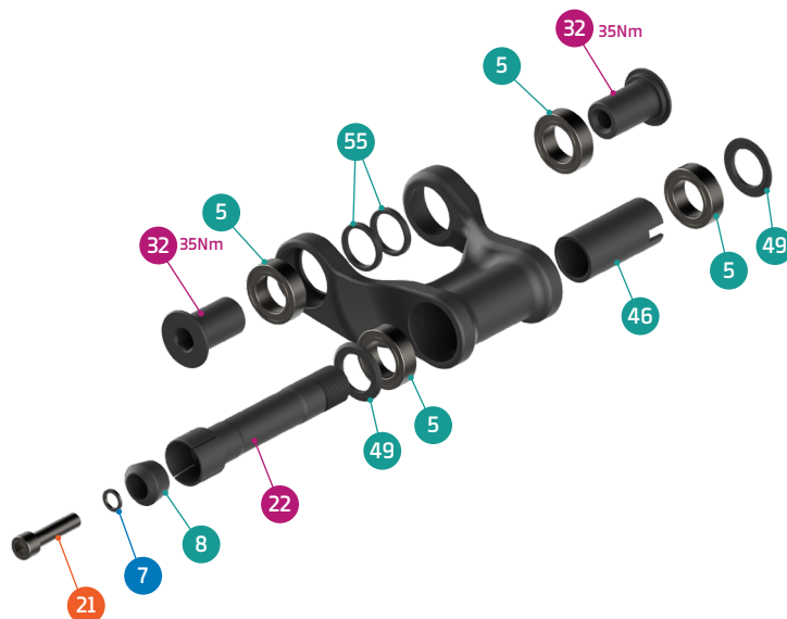
DETAIL 02
