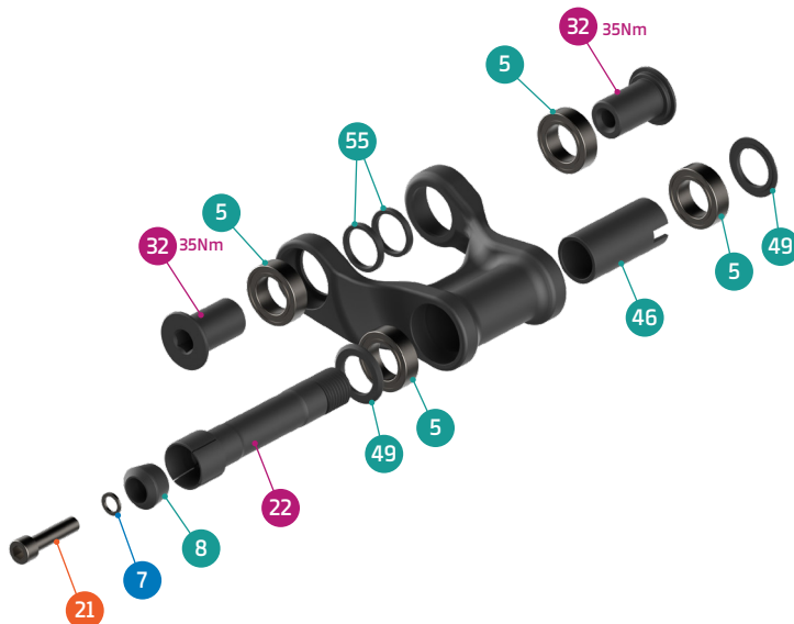
DETAIL 02
