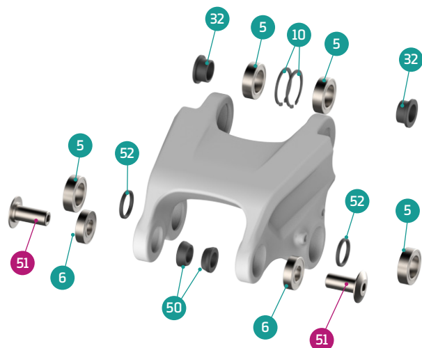
DETAIL 01
