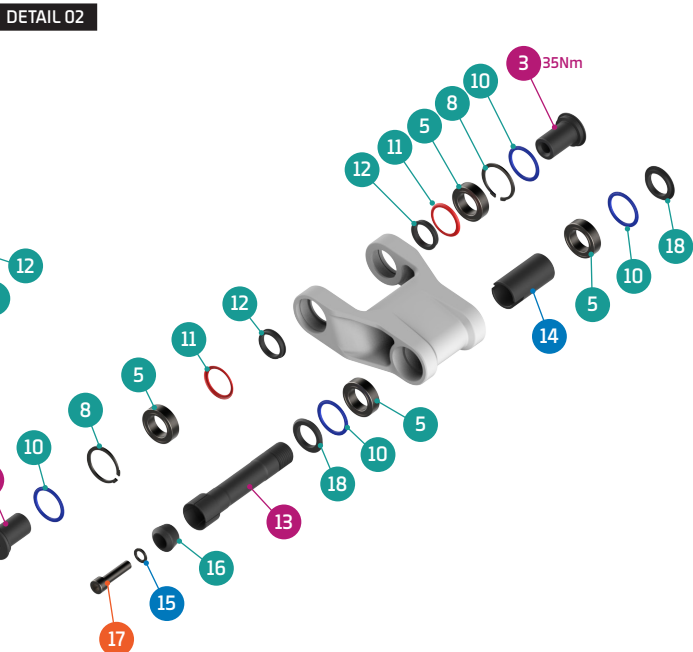
DETAIL 02
