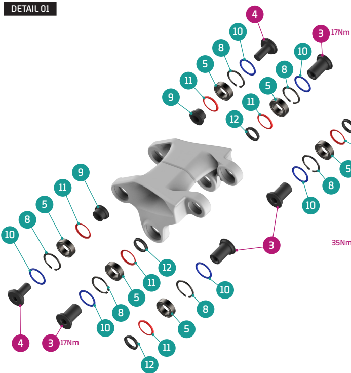
DETAIL 01
