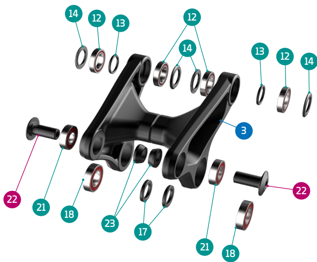
DETAIL 01
