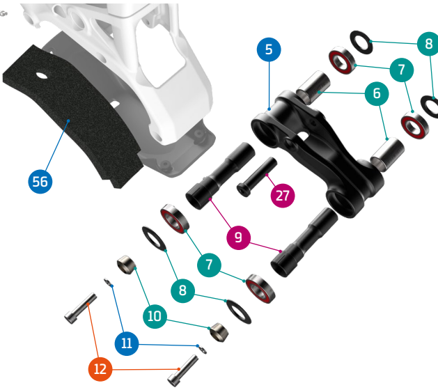
DETAIL 02
